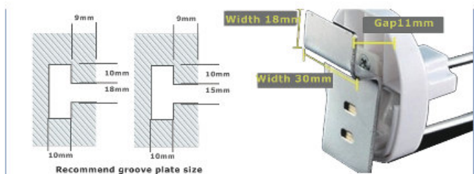
SF2002-Groove Plate
