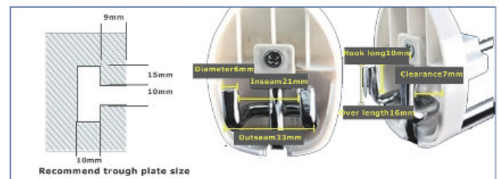
SF2001-Slot Plate
